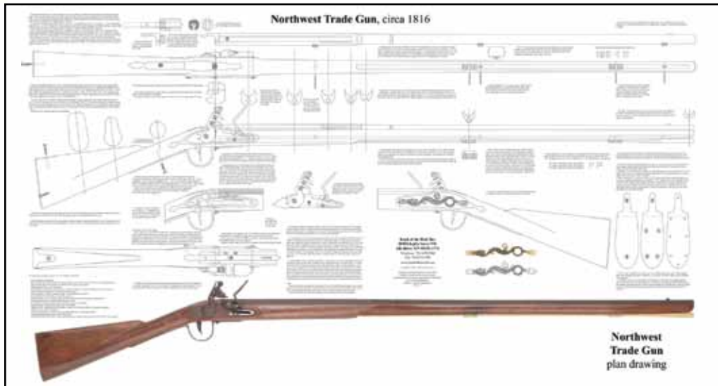
Northwest Trade Gun by Forrest Grilley using Track's best parts and plan drawing.
